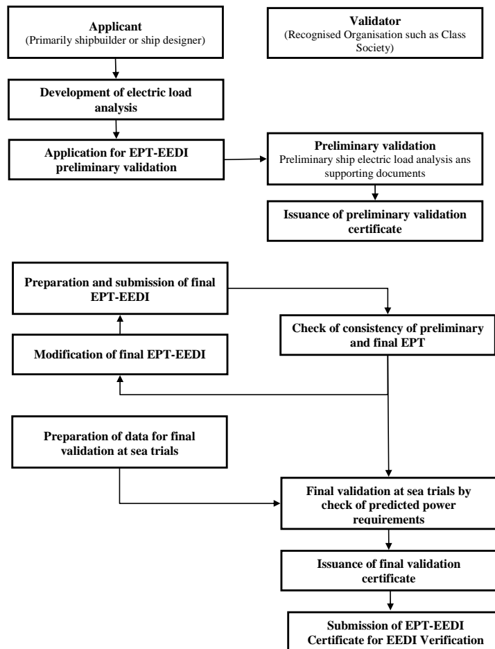
Figure 1 - Basic Flow of EPT-EEDI Validation Process
